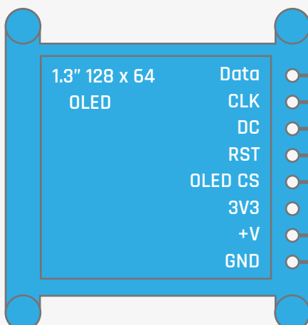
Fig 1 Connecting the OLED display to the Raspberry Pi
