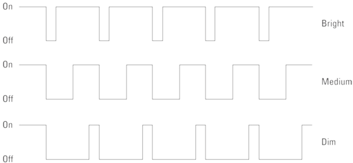
FIGURE 17-3: A PWM signal controlling the LED's brightness.
