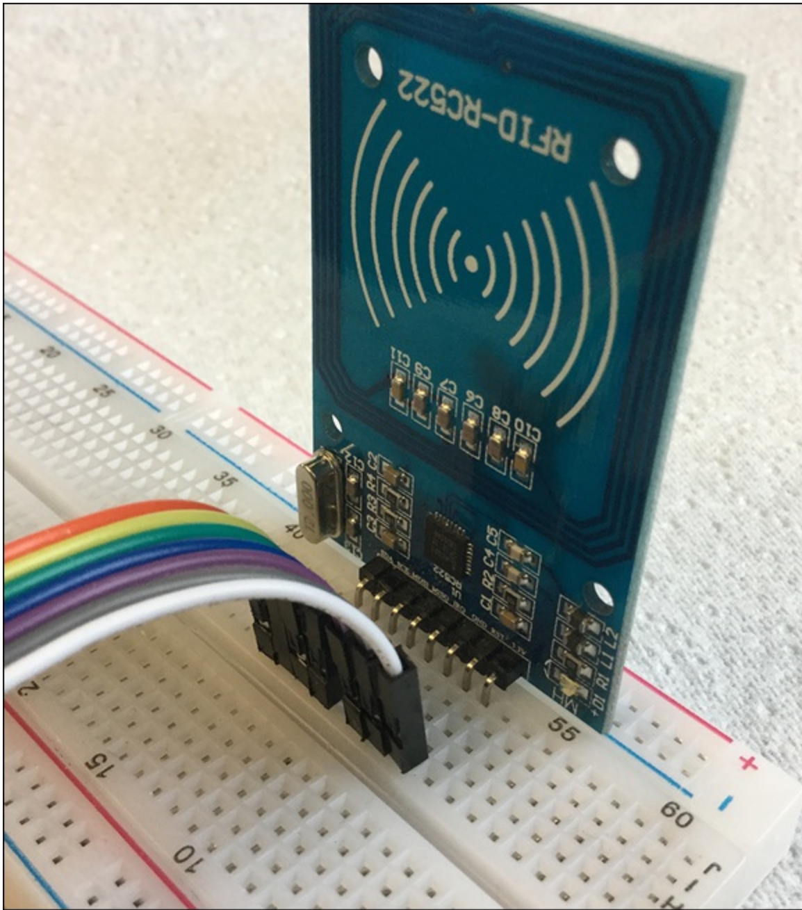
FIGURE 18-2: Mounting a reader on a breadboard.
