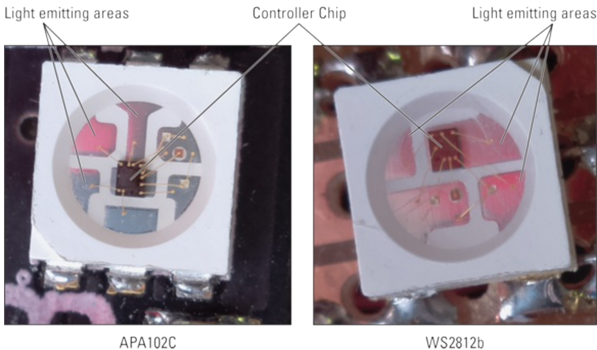
FIGURE 17-4: DotStar (APA102C) and NeoPixel (WS2812b) LEDs.
