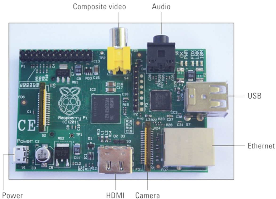
FIGURE 3-1: The original Model B Raspberry Pi. The Model A is the same, except that it has no Ethernet.
