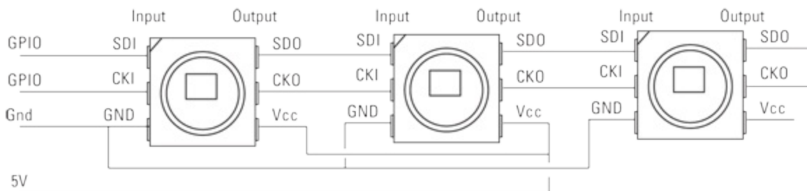
FIGURE 17-5: Wiring of an APA102C LED chain.
