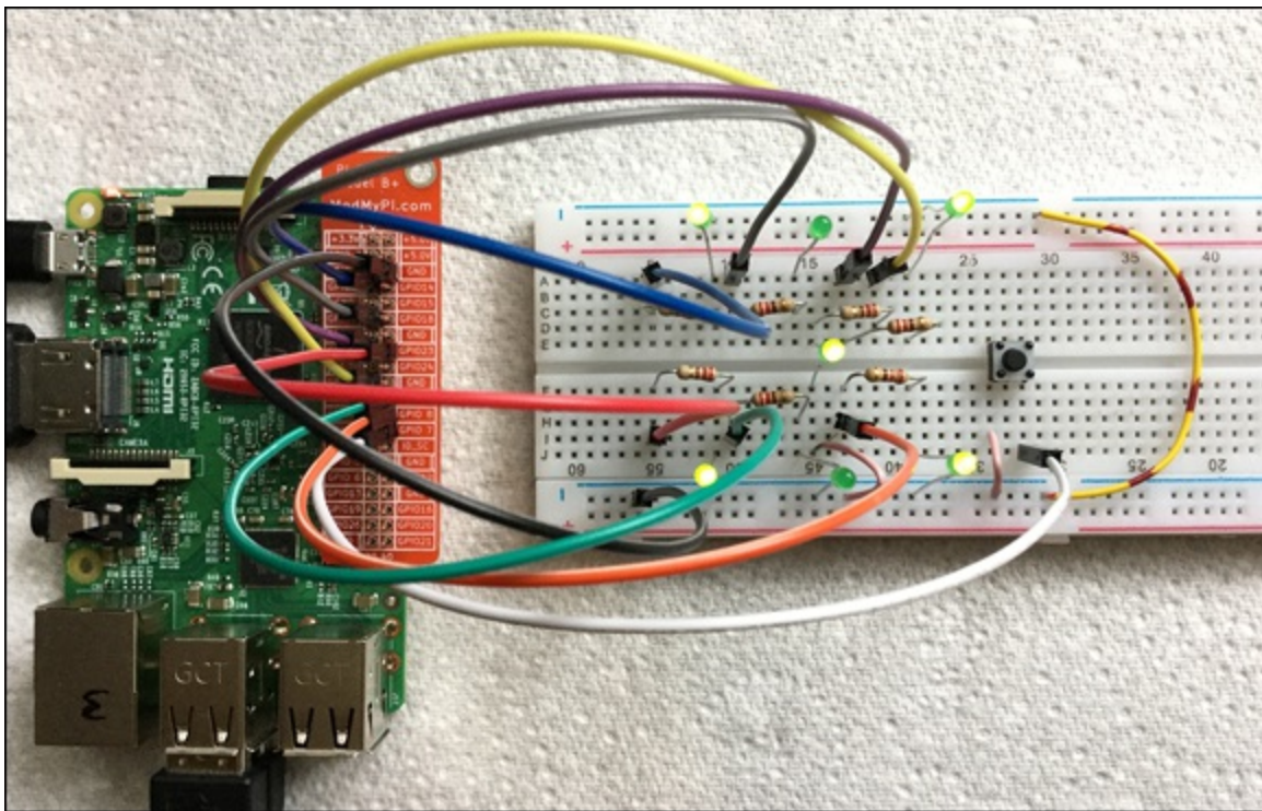
FIGURE 16-11: Photo of the LED dice project.
