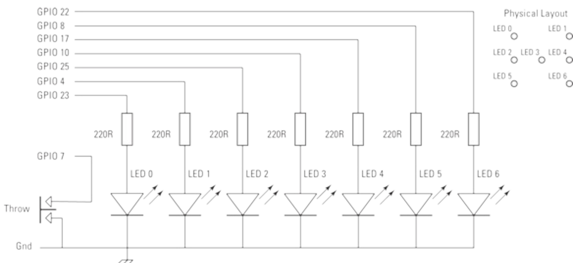
FIGURE 16-9: LED dice schematic.
