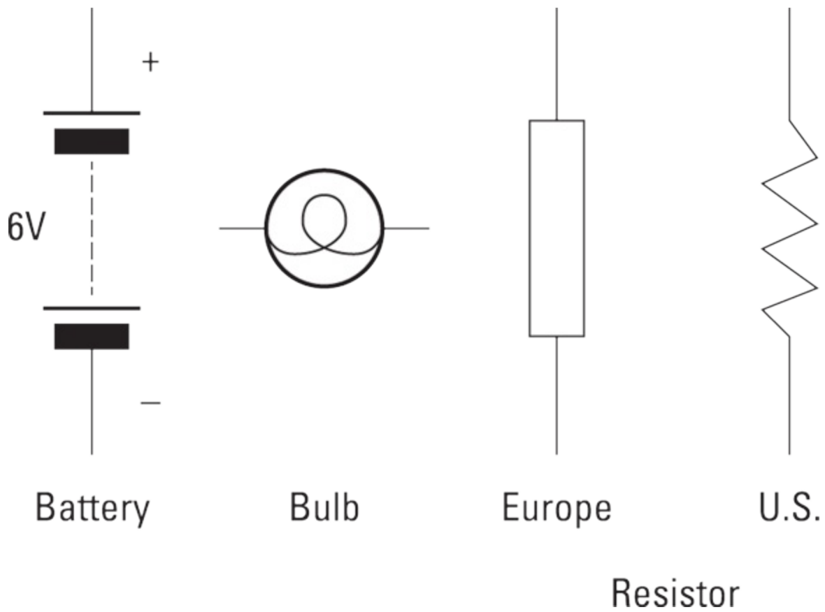
FIGURE 15-3: Schematic symbols for some components.
