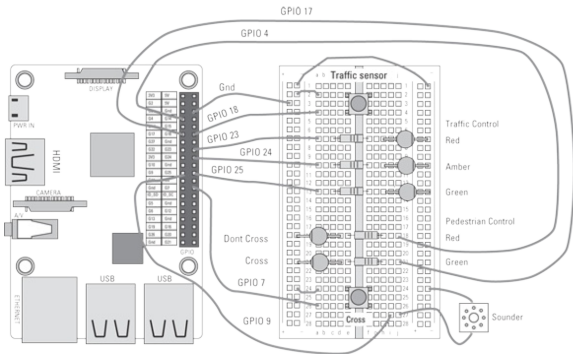
FIGURE 16-15: Layout of the Traffic Crossing circuit.
