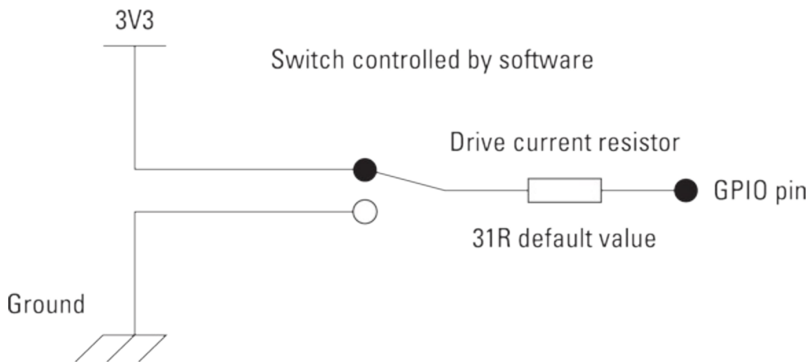
FIGURE 15-7: A GPIO when used as an output.
