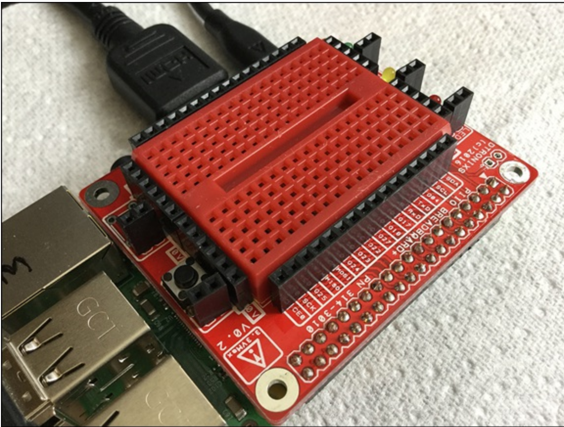
FIGURE 16-5: The Dtronix combined bread-board-and-shield.
