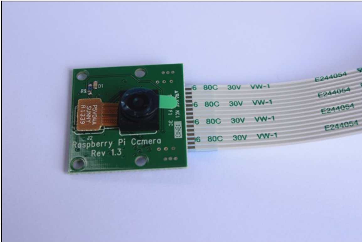
FIGURE 3-7: The Raspberry Pi Camera Module.
