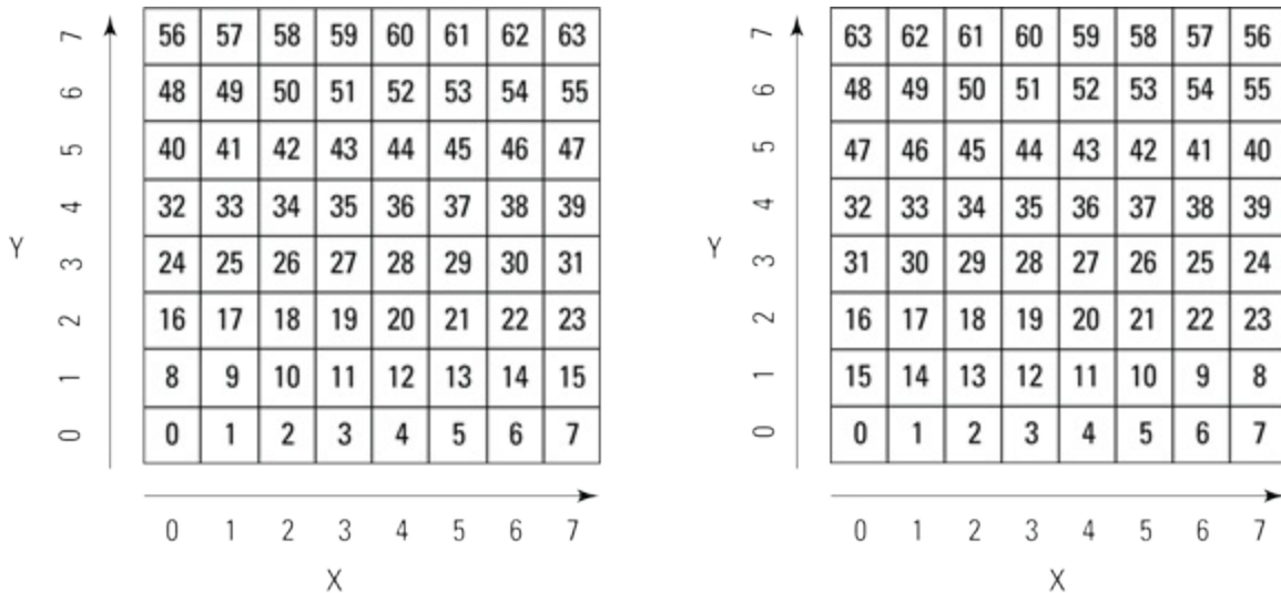
FIGURE 17-12: Making a matrix with raster wiring and serpentine raster wiring.
