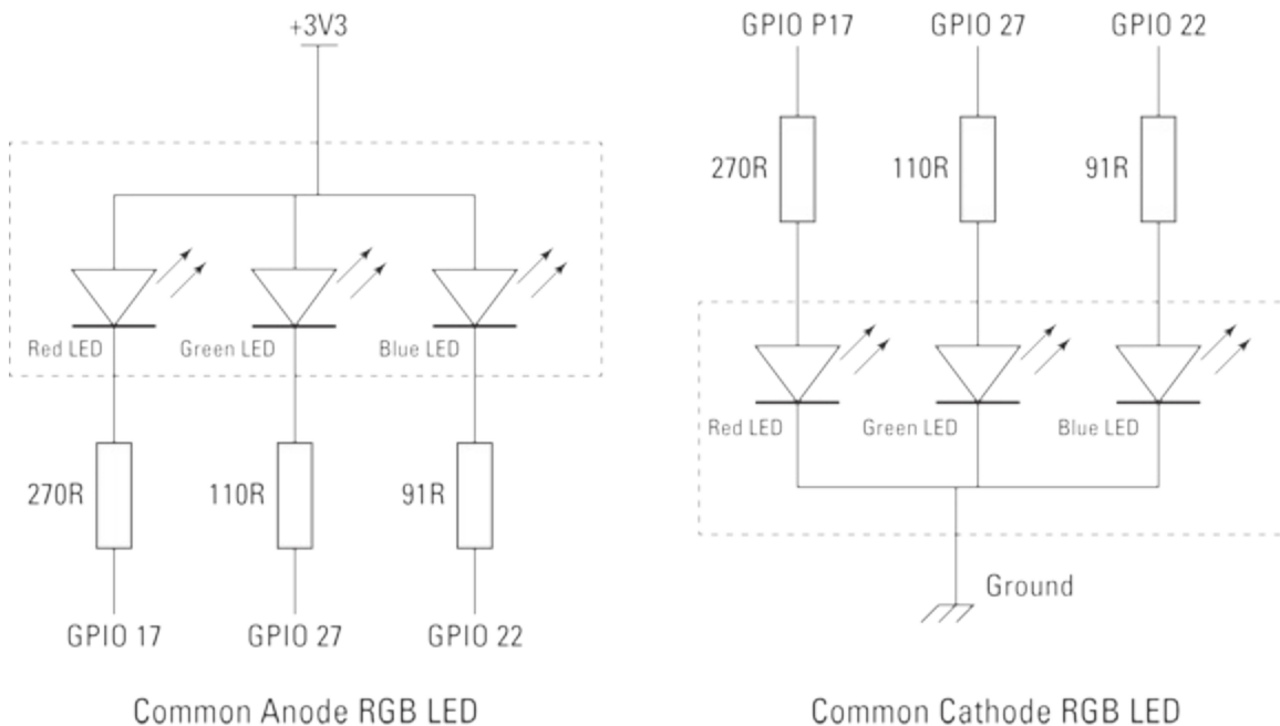
FIGURE 17-2: Wiring common anode and common cathode LEDs.
