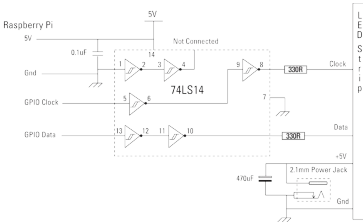
FIGURE 17-9: APA102C driver circuit.
