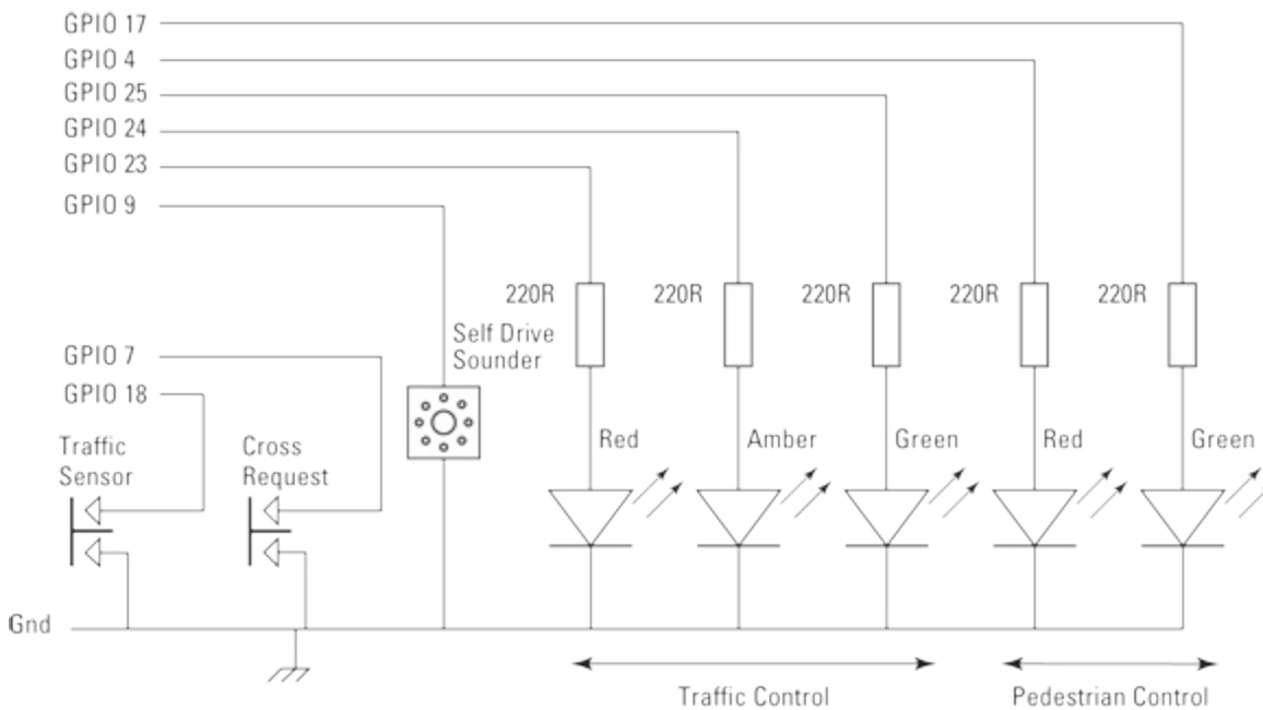
FIGURE 16-14: Pedestrian Crossing schematic.
