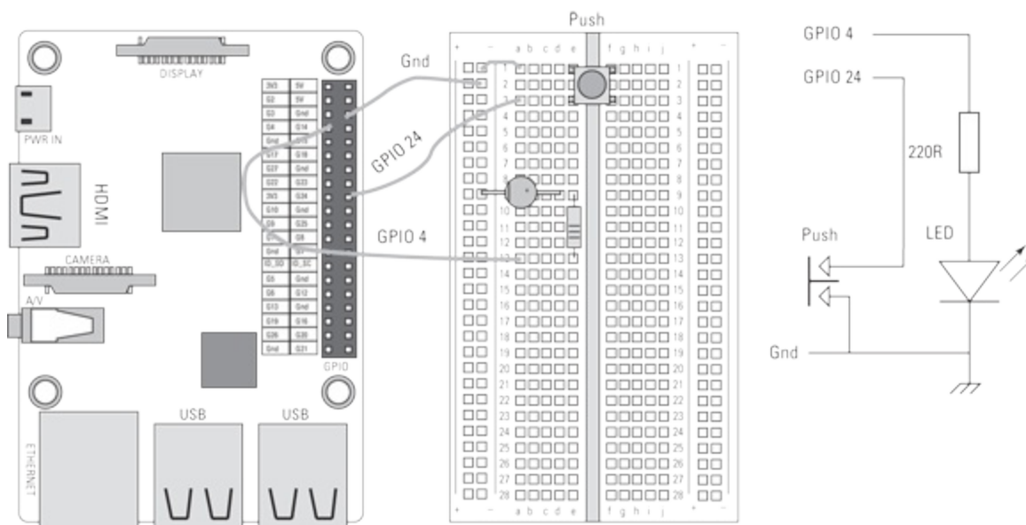
FIGURE 16-6: An LED and switch, wired to the GPIO pins.
