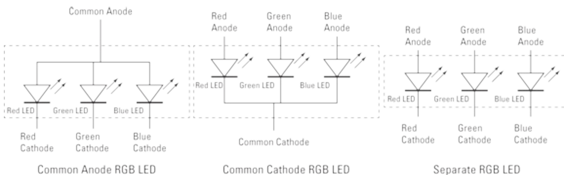
FIGURE 17-1: Three types of basic RGB LEDs.
