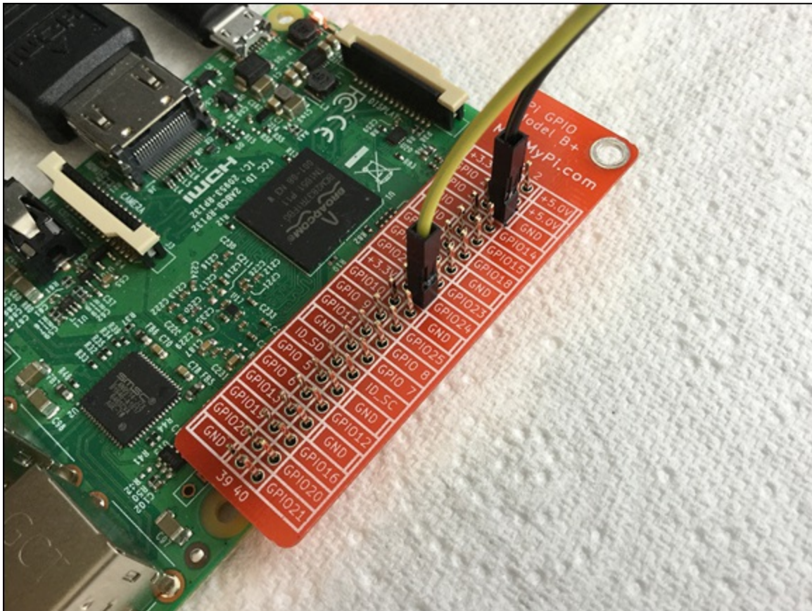
FIGURE 16-2: GPIO template identifying the pins.
