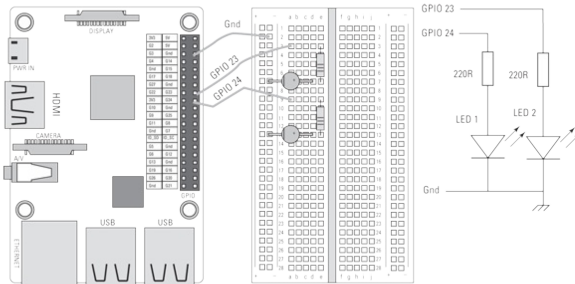
FIGURE 16-13: LED wiring for independent blinking.
