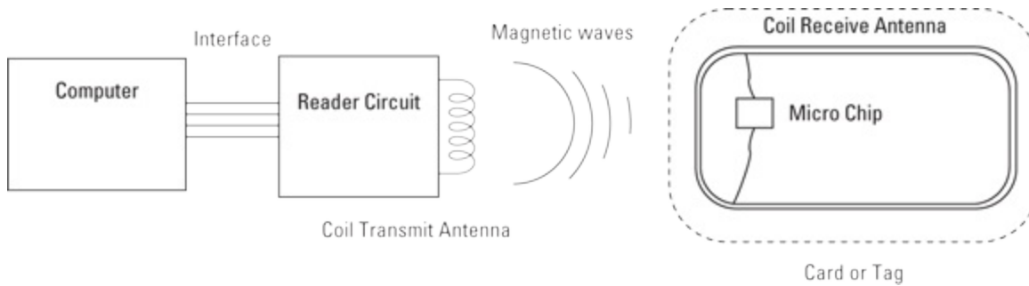
FIGURE 18-1: Block diagram of an RFID system.
