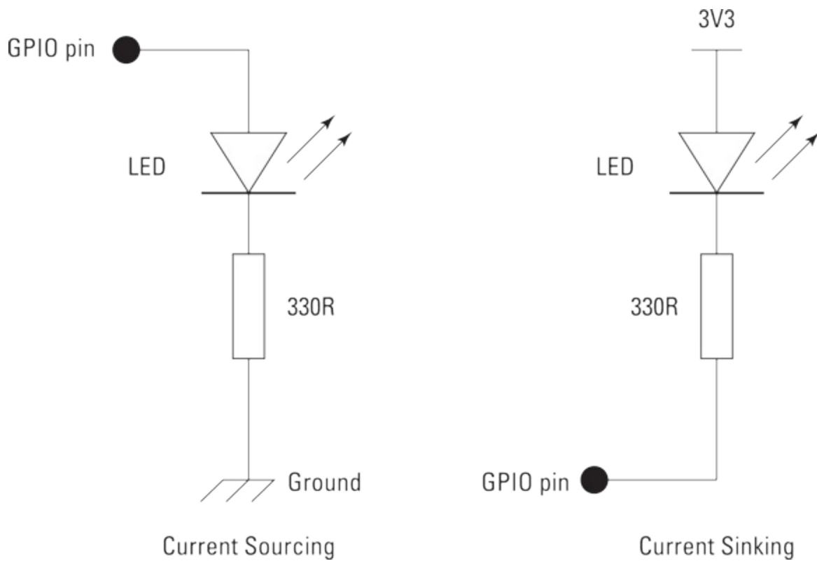
FIGURE 15-8: Two ways of driving an LED.
