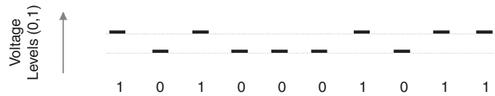
FIGURE 1-10 Binary Digitalization
